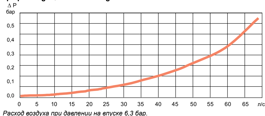
График. ErgoQIC 10 M15 и ErgoNIP 10 M15
