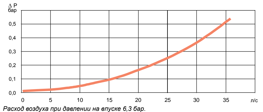
График. ErgoQIC 10 ASIA и ErgoNIP 10 ASIA
