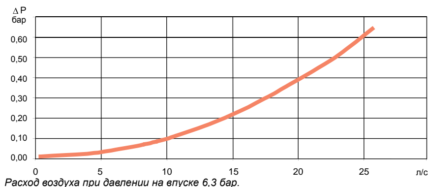
График. QIC 10S M10 и NIP 10 M10
