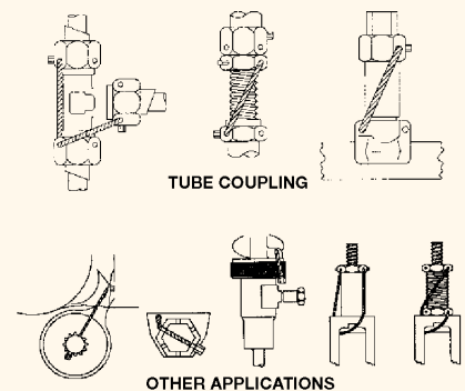
FIGURE 9: Examples of Installed Safe-T-Cable®
